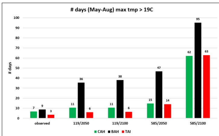
Figure 14. The number of days > 19°C in each scenario.
